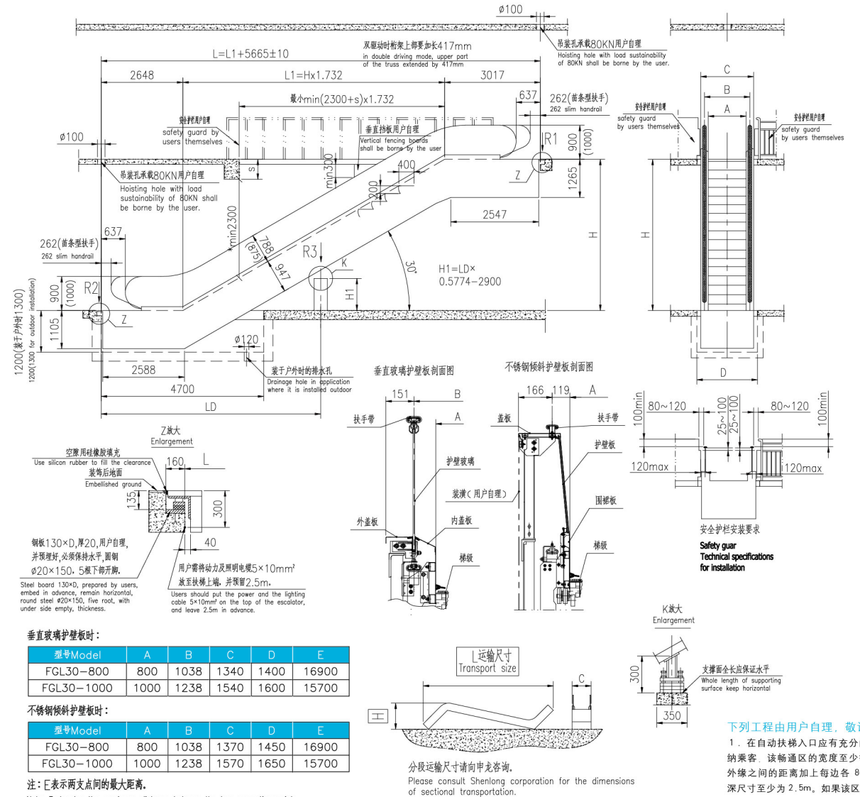
30°FGL Public Traffic Type Escalator Construction Layout
