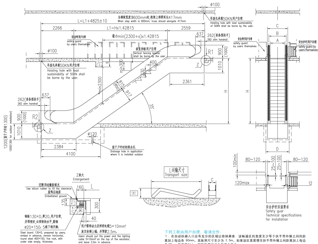
35° FPL Common Type/FML Slim Type Escalator Construction Layout
